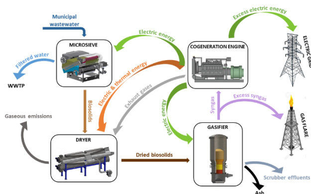
Σχήμα 1. Mass and energy flows of biosolids microsieving-gasification pilot plant.
